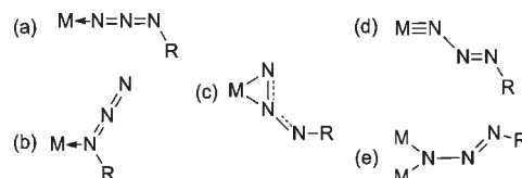
Scheme 2. Coordination Modes of Organic Azides: (a) Terminal Azide Nitrogen ( \text{N}_\gamma ) Complexation; (b) Coordination through \text{N}_\alpha ; (c) \eta^2 -Adduct Analogue of Olefin Complexation; (d) Diazenimido and (e) Bridging \mu -Imido Ligand
