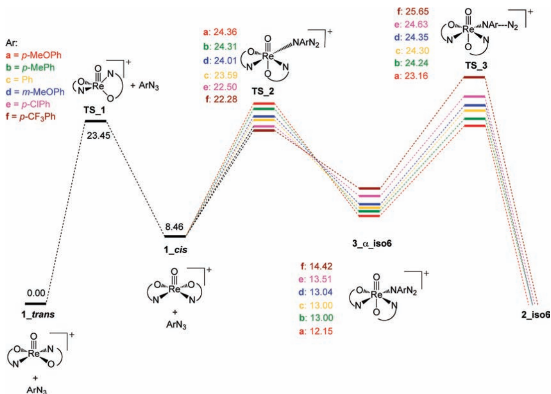
Figure 6. Solvated \Delta G ( \text{kcal mol}^{-1} ) diagram for the reaction of the rhenium oxo complex with \text{ArN}_3 (solvent: \text{CH}_3\text{CN} ).
