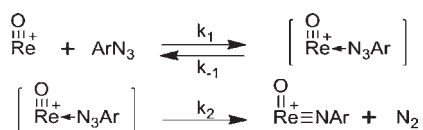
Scheme 6. Proposed Kinetic Mechanism for the Reaction of ArN 3 with 1
