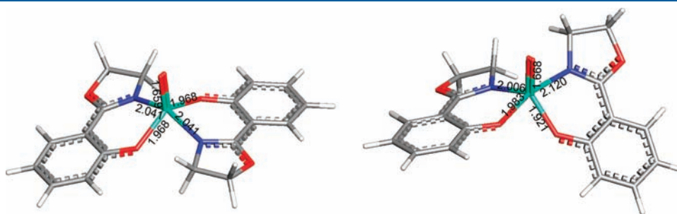
Figure 4. Structures and some selected bonds lengths of 1 trans (left) and 1 cis (right). The ligands lying in the equatorial plane are relatively flat in 1 trans and fairly twisted in 1 cis .
